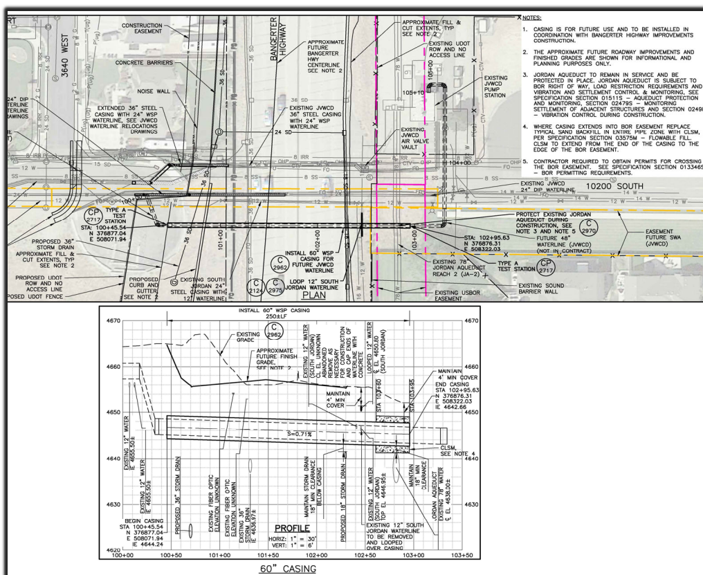
Plan sheet from the 60" casing crossing Bangerter Highway
