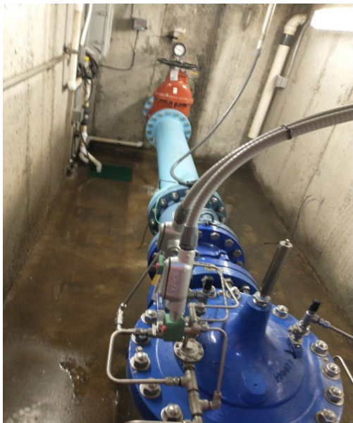
New pipeline, meter, and valves
