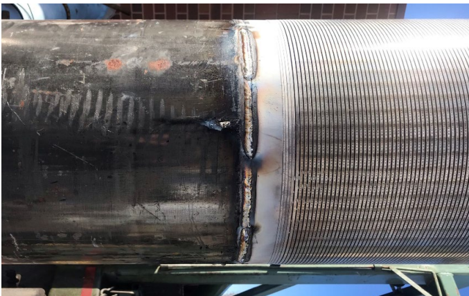
Welded joint, transitioning from stainless steel screens to steel casing.
