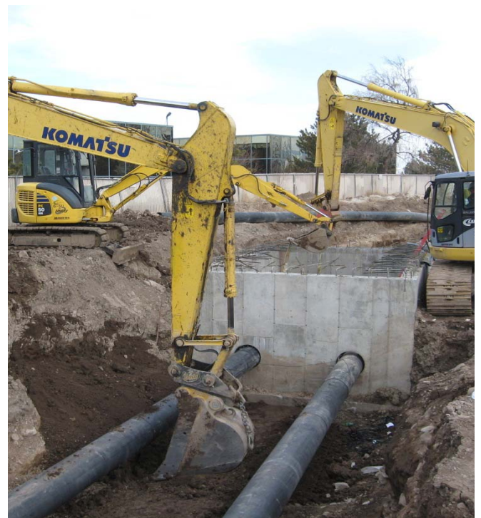
Construction of Intermediate pig Vault at 8400 West along the U&SL Canal
