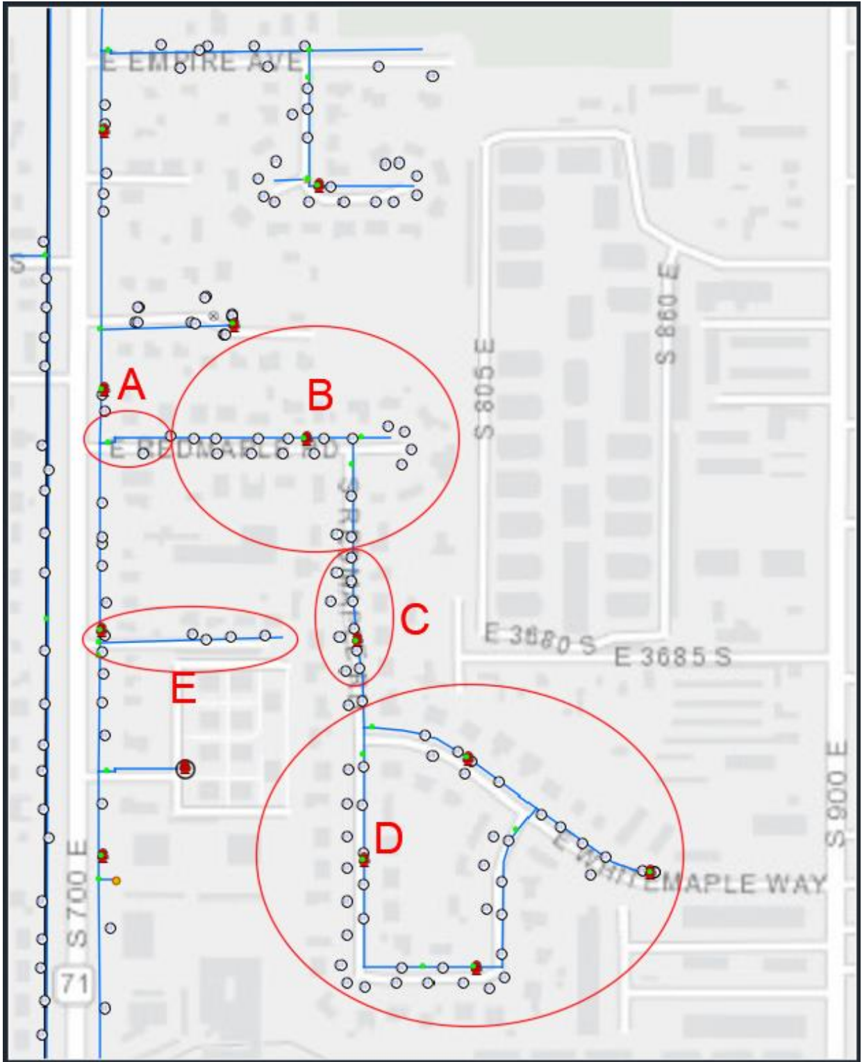
Figure 1: Areas of new Distribution Pipeline in Redmaple Area
