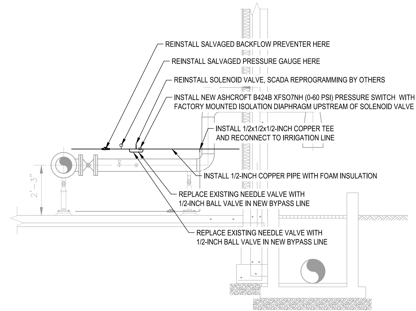
B-B' SECTION VIEW SCALE: SCALE
