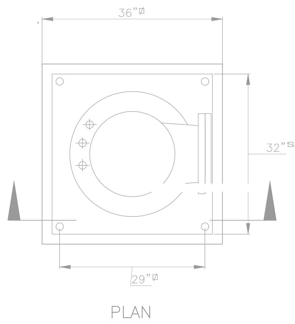
DW 6 WELLHEAD CONFIGURATION SCALE: NONE
