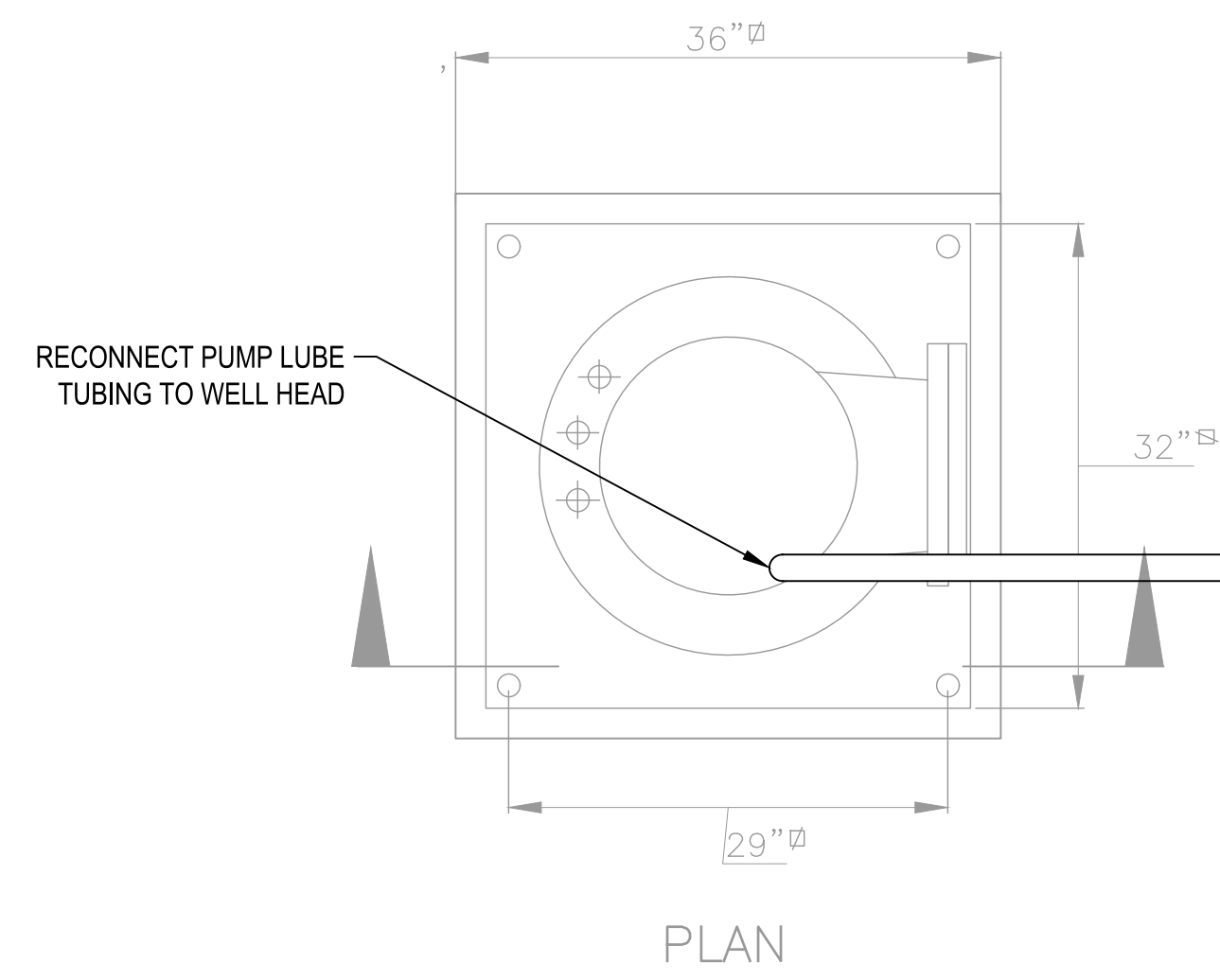
CU104 DW 6 WELLHEAD CONFIGURATION SCALE: NONE
