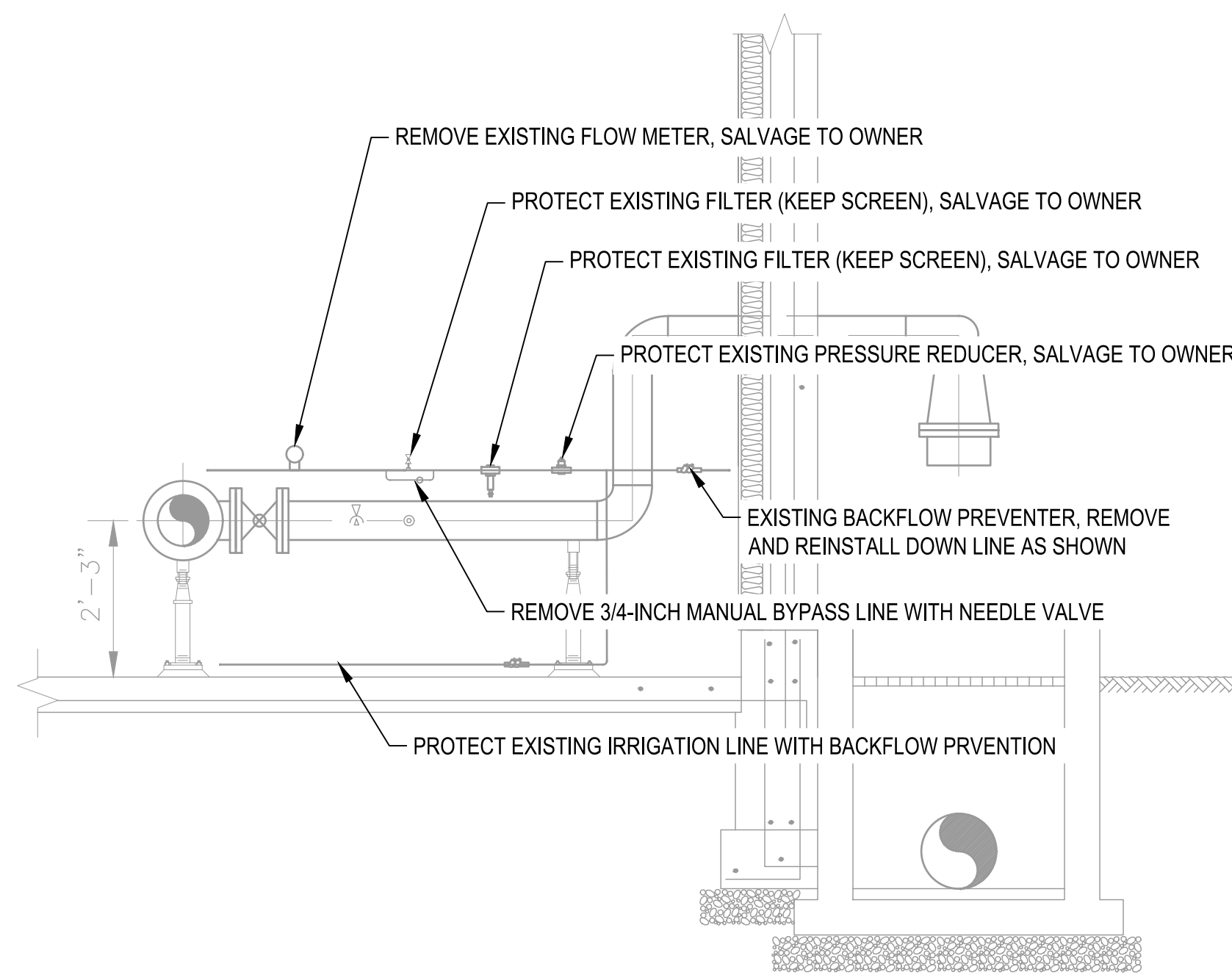
B-B' SECTION VIEW SCALE: SCALE
